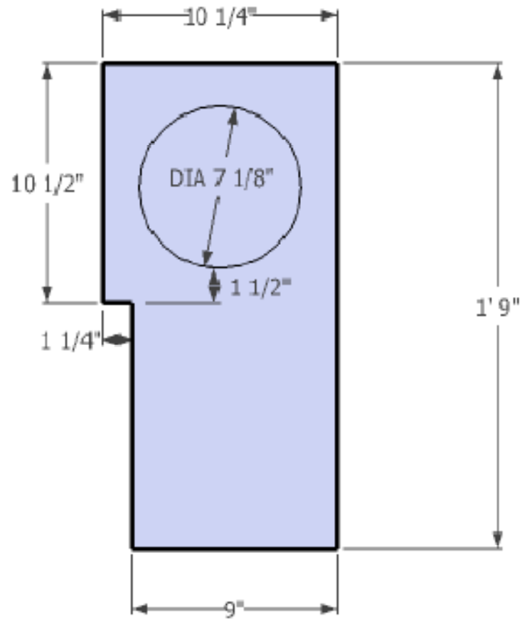
FRONT DIMS
