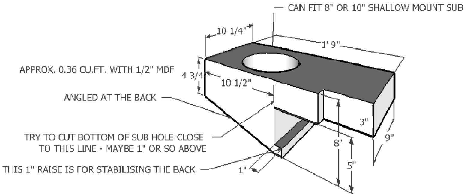
SIDE DIMS
