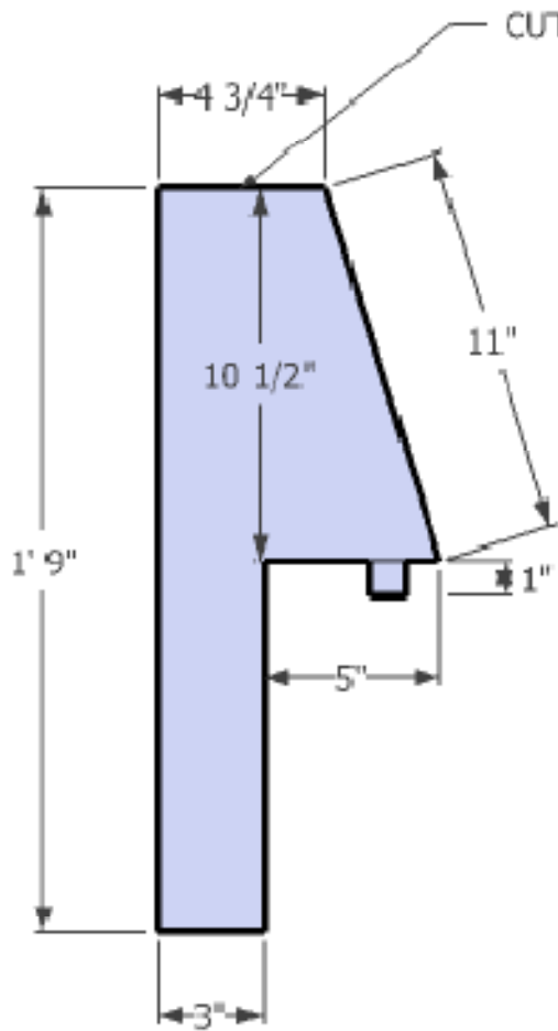
SIDE DIMS
